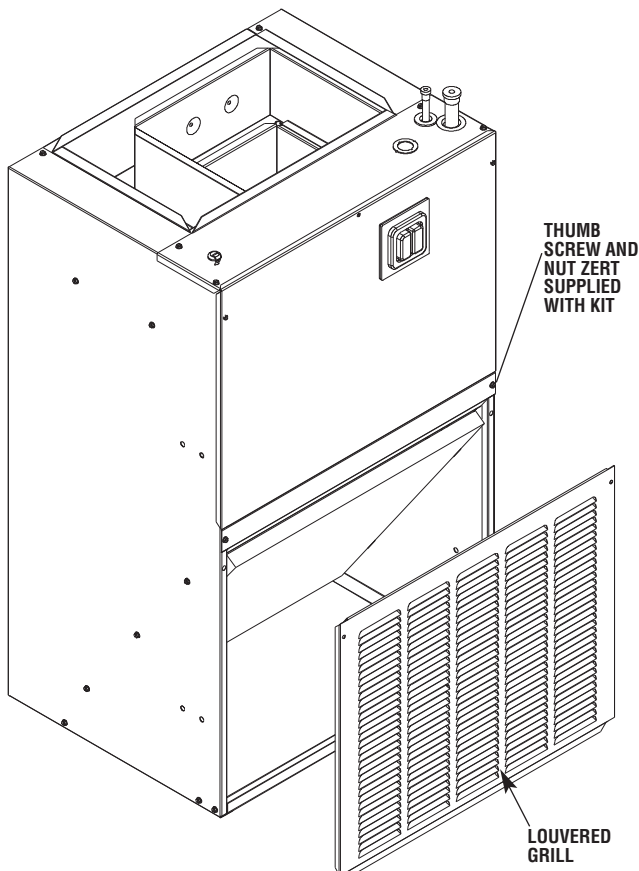
FIGURE 1 UNIT ASSEMBLY INSTRUCTIONS
