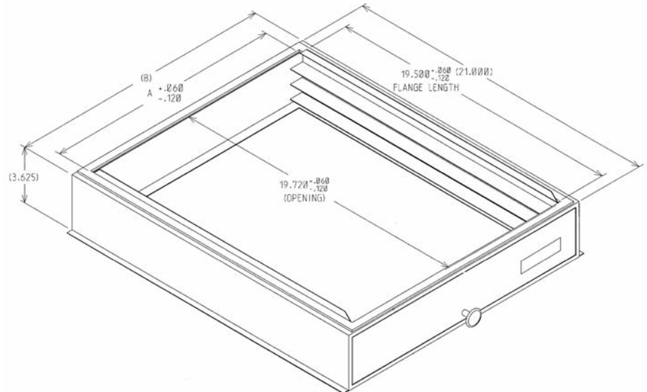
FIGURE 30 EXTERNAL FILTER BASE: RXHF-
