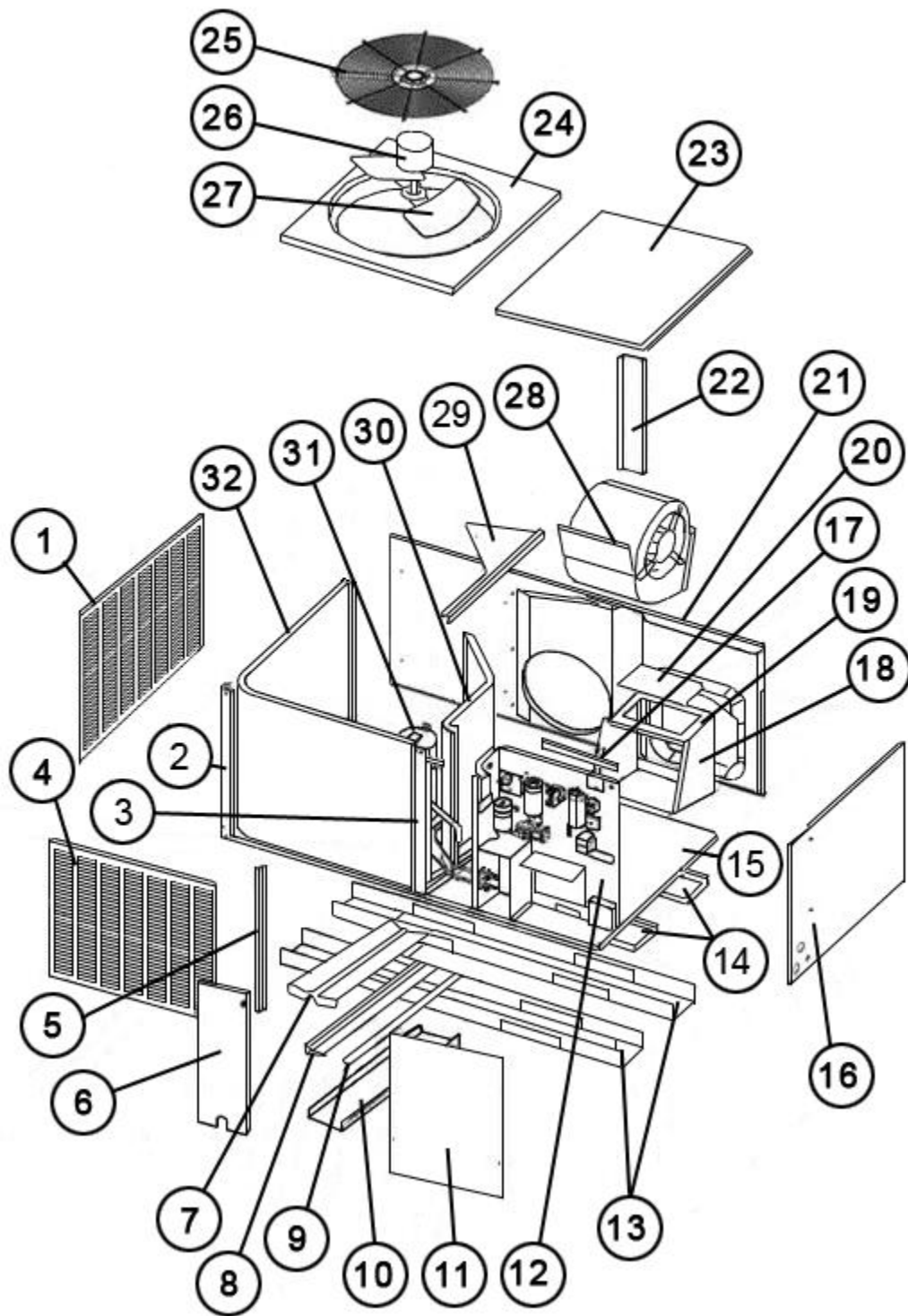
Exploded View
