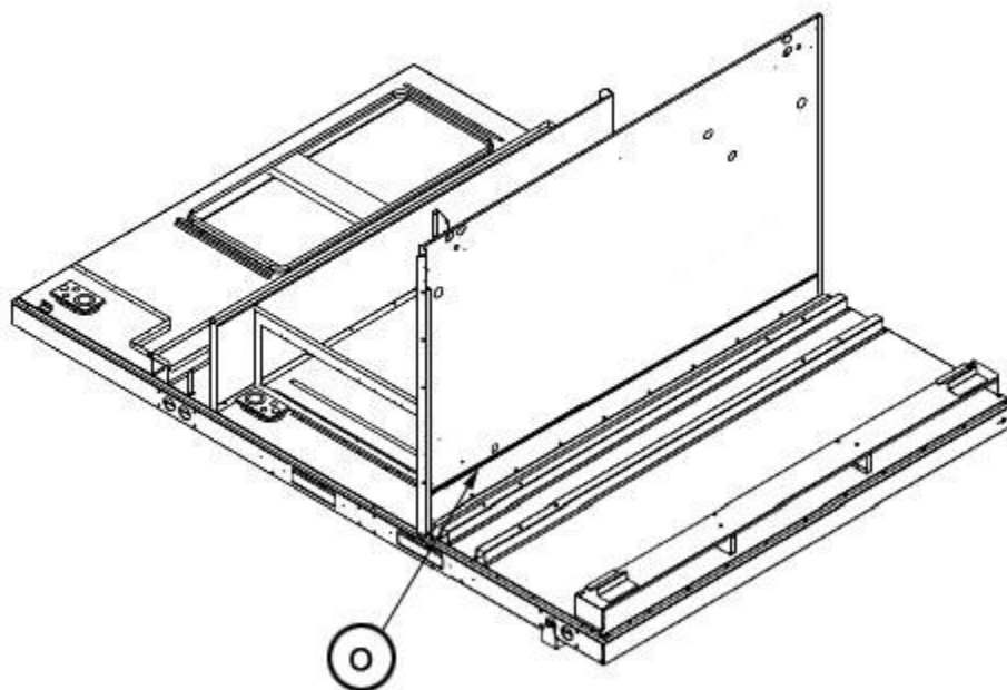
Condenser Bulkhead 180-240
