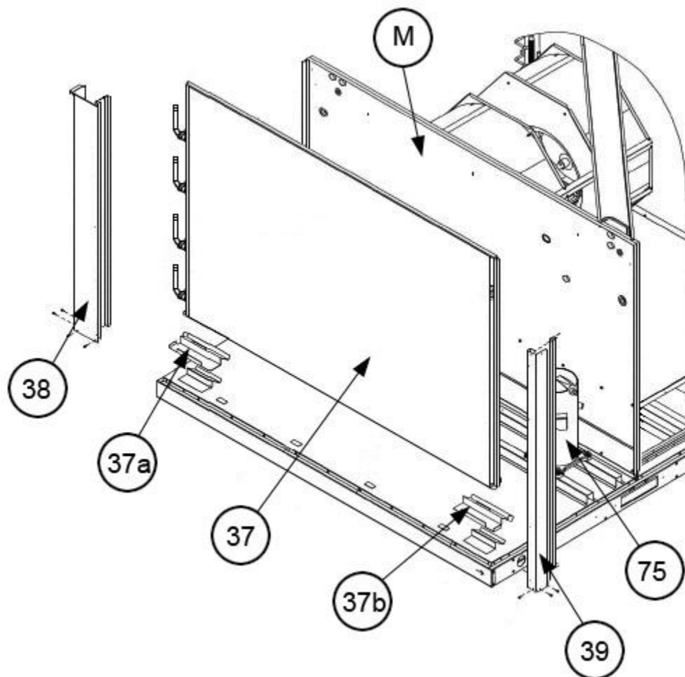
Condenser Coil 180
