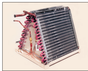
Indoor Coil - Copper Tube / Aluminum Fin Design
