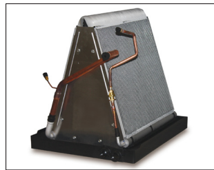
Indoor Coil - Microchannel (All Aluminum) Construction
