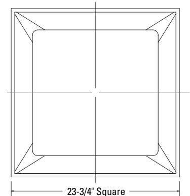
4750-6 AL Face View
