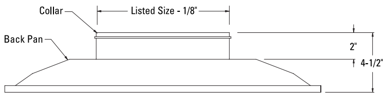
4750-6 AL: Plaque Ceiling Diffuser - T-Bar - Steel
