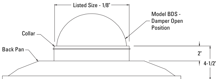
Option: 4750-6 AL BDS: Plaque Ceiling Diffuser - T-Bar - Steel - w/ BDS Damper
