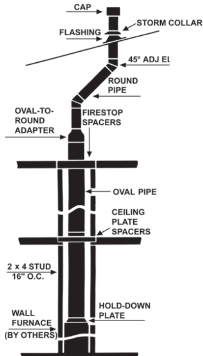
Type BW Gas Vent
