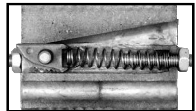
Cutaway inside view of lock
