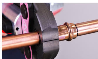
2. Complete the joint with the approved tool. Press once only
