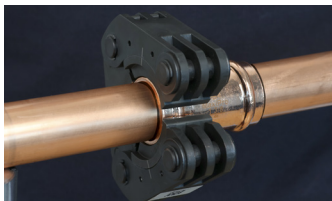
1. Fit the pressing ring
