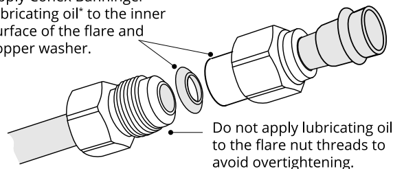
Stainless flare with copper washer
